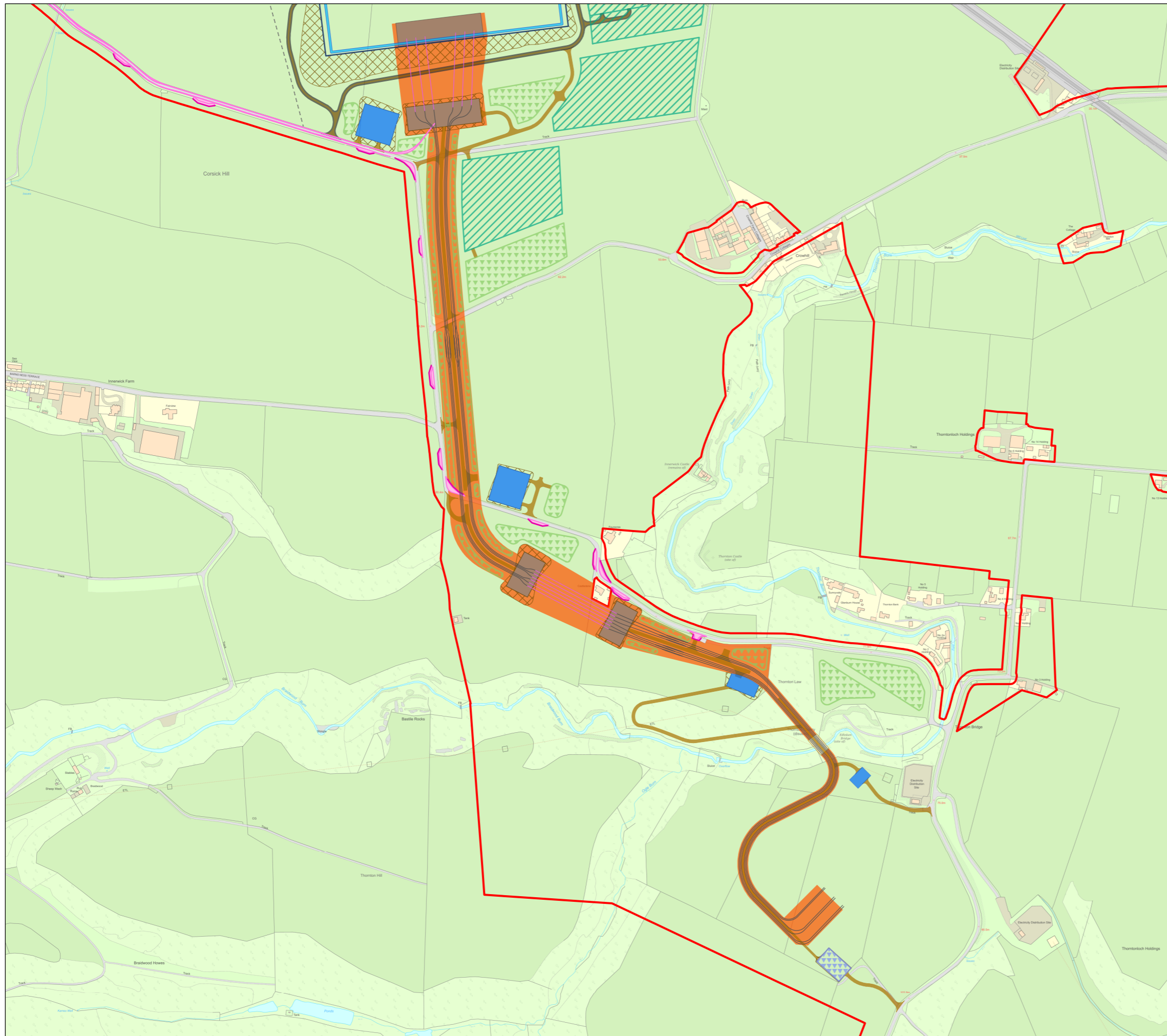
Drawing Title FIGURE 5.4 SITE LAYOUT ELECTRICITY TRANSMISSION BUILDINGS TO GRID CONNECTION
